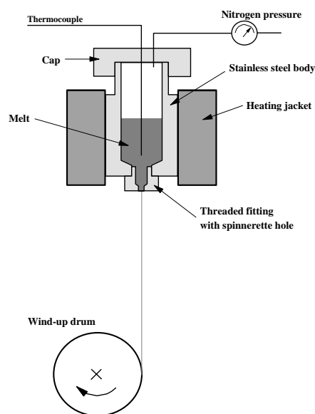
Fig. 1: A single hole spinnerette
