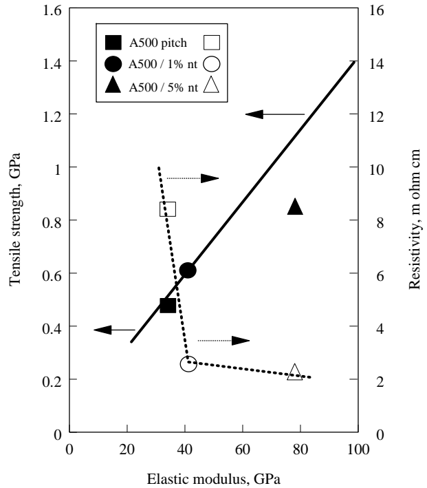
Fig. 2 Experimental values of properties of nanotube-pitch composite carbon fibers.
